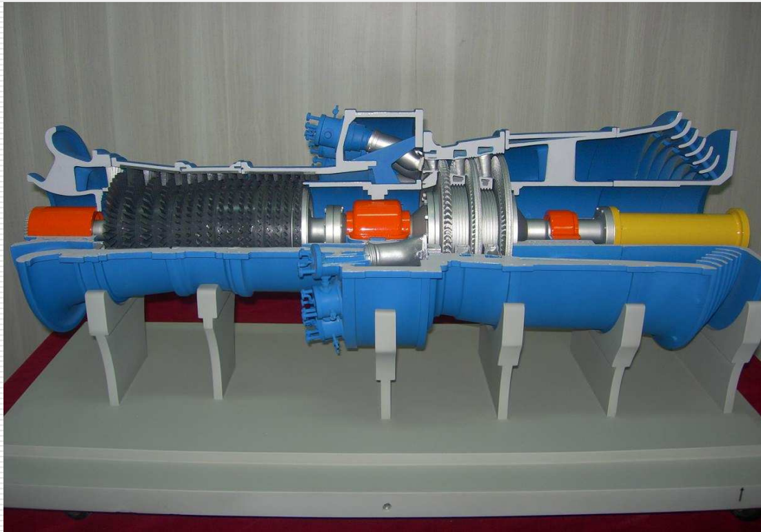
Cut sectional, 16 component Micro model of Gas Turbine
